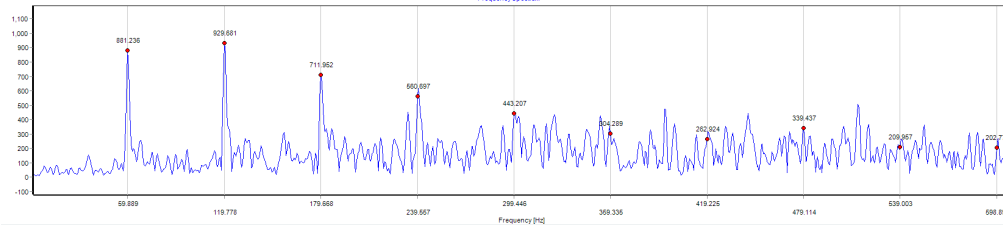
Figure 2 FFT Shows the 1st, 2nd, 3rd and 4th occurrence of a 60 Hz Harmonic Marker indicating the Critical Angle was achieved for this anomaly.
