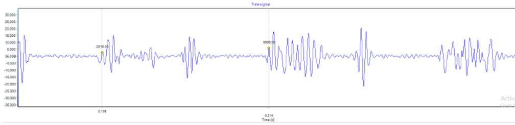
Figure 6 A Period of 0.167 seconds clearly shows up in the Time Series.
