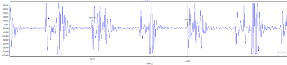
Figure 1 Time Signal clearly shows peaks within 0.0167 seconds which indicates 60 Hz
